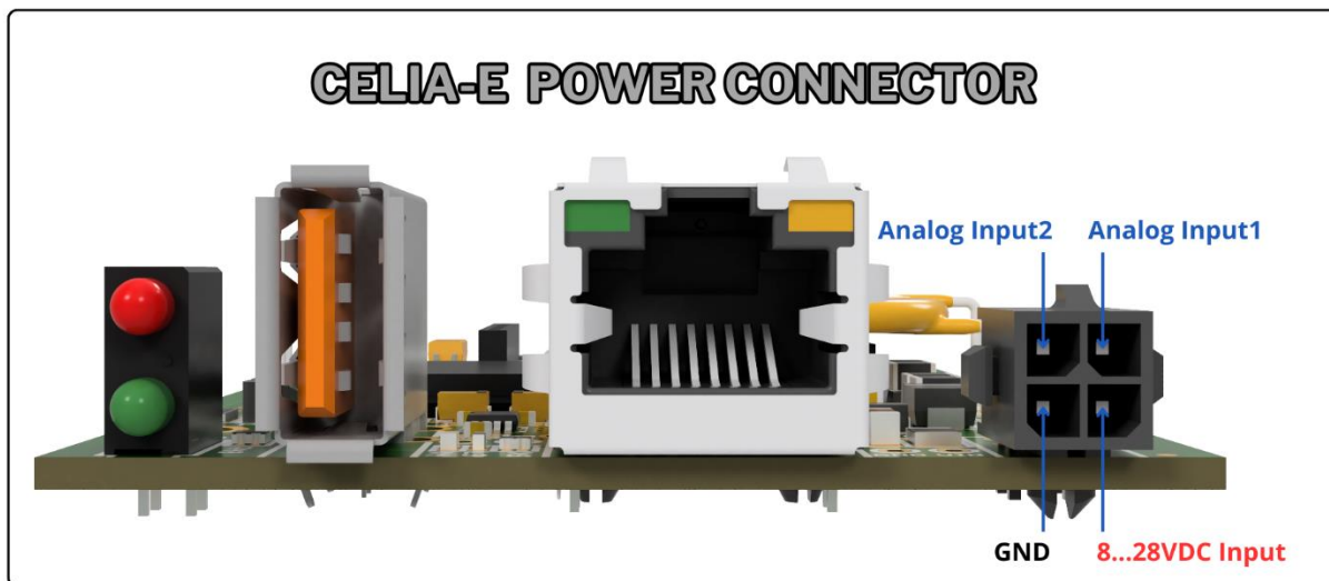
Figure 2: Diagram of connections for power supply cable connector.
