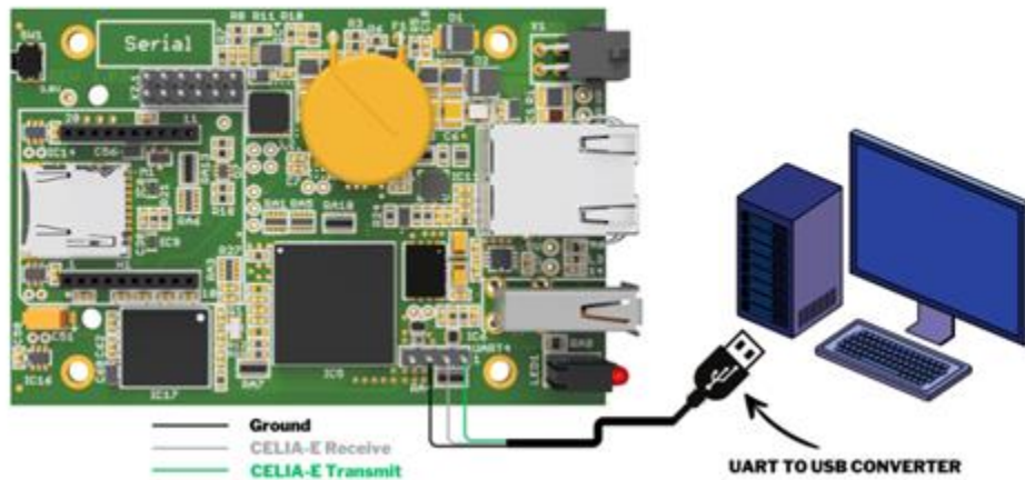
Figure 4: UART connections
